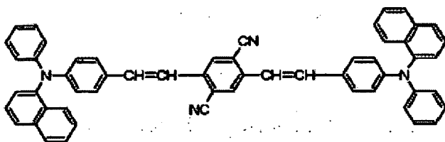
Structural formula (15)-11:
